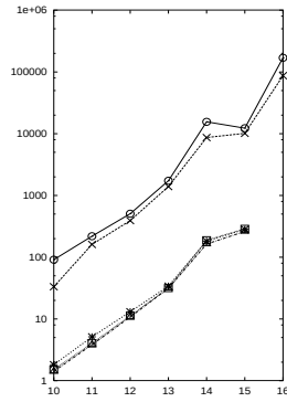
Fig. 22. stack, prop. 1, weak
