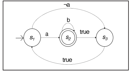
Fig. 4. Non-monitorable automaton
