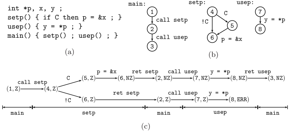
Fig. 1. (a) An example program, (b) its function CFGs, and (c) the derivation graph
