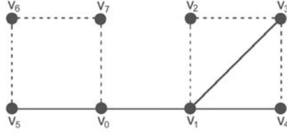
Fig. 2. The Equality Graph G^E(\varphi^E) corresponding to the non-polar version of the same graph shown in Figure 1
