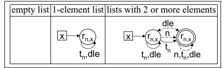
Fig. 7. The structures that describe possible inputs to InsertSort
